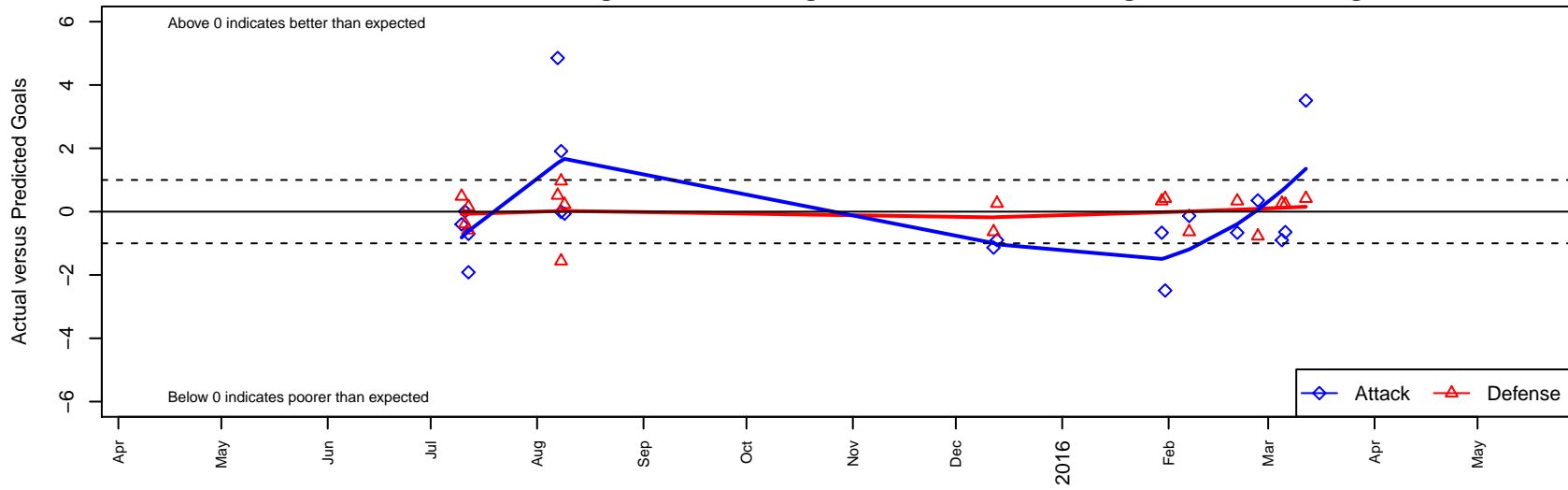
SSC Shadow B G97 Dots are actual minus expected GF (blue circles) and GA (red triangles). Blue line is smoothed change in attack strength. Red is smoothed change in defense strength.
